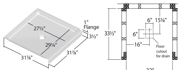
3232 Elite™ CTR Drain (LEBxx3232)
