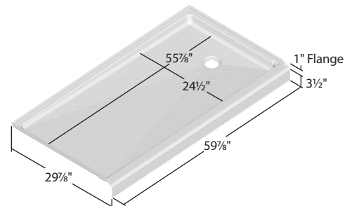
6030 Stud Layout RH drain shown Opposite for LH drain
