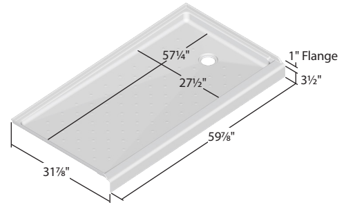
6032 Stud Layout RH drain shown Opposite for LH drain
