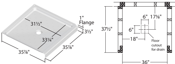
3636 Stud Layout ⊠ = required stud location ⊠ = suggested stud location
