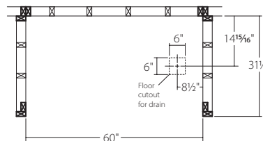
3232 Elite™ CTR Drain (LEBxx3232)
