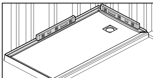
FIGURE 2. Check to assure base is level.
